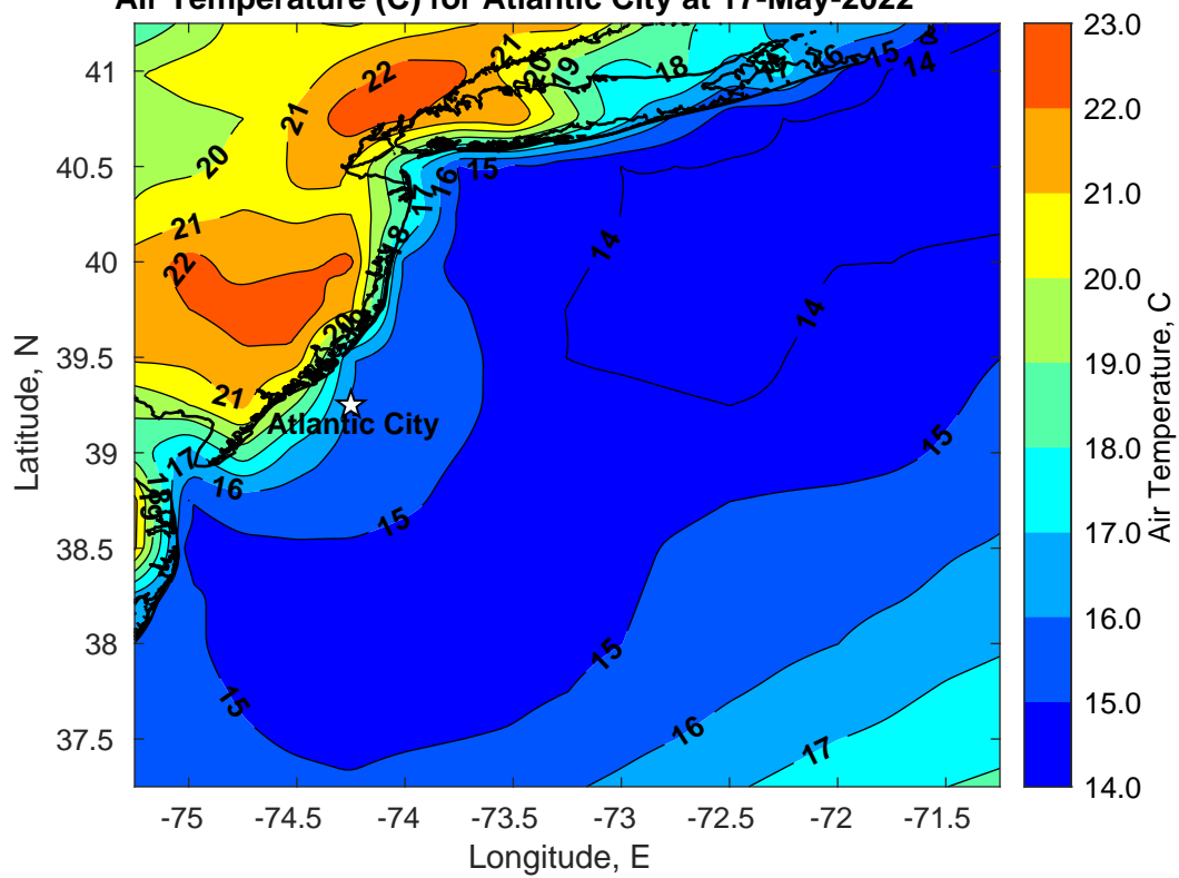
Air Temperature (C) for Atlantic City at 17-May-2022
